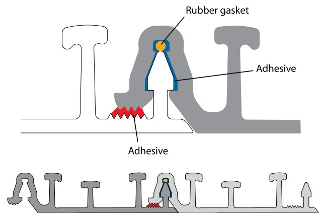
Cross-section of typical Rotaloc profile, showing the mechanism that locks together successive wraps of profile.
